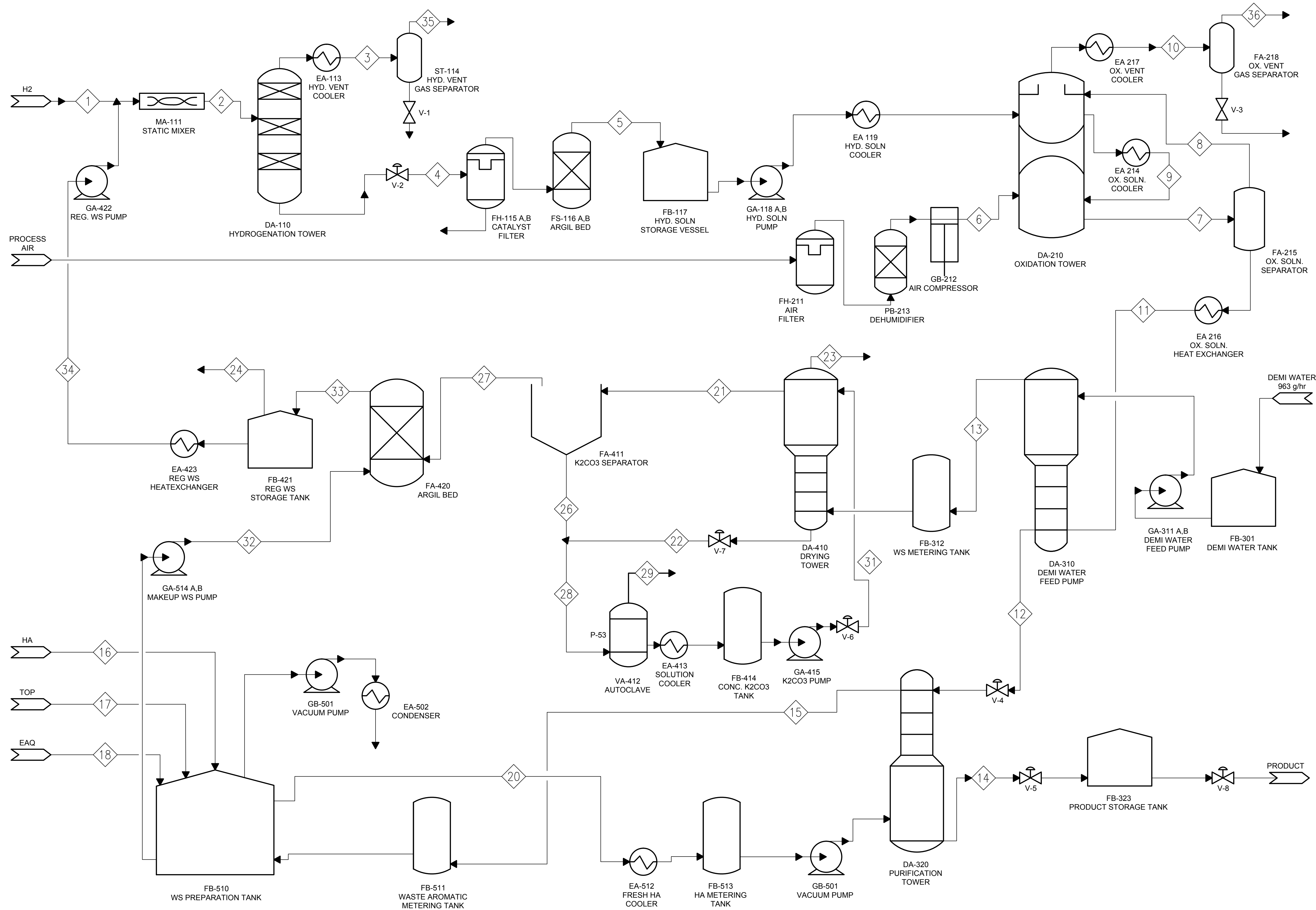
PROCESS FLOW DIAGRAM FOR HYDROGEN PEROXIDE PLAN
