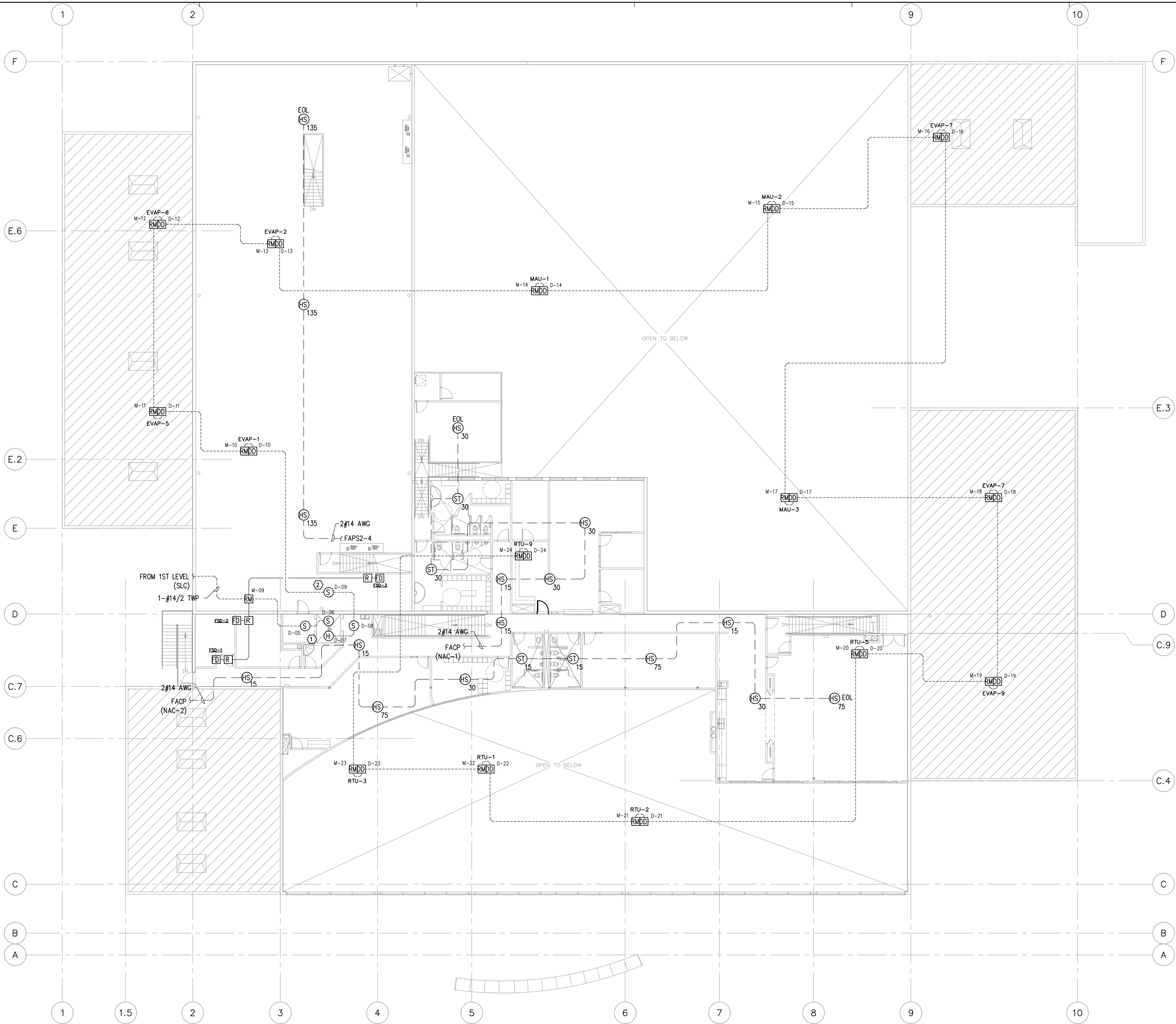
2ND LEVEL SCALE: 3/32" = 1'-0" FIRE ALARM PLAN
